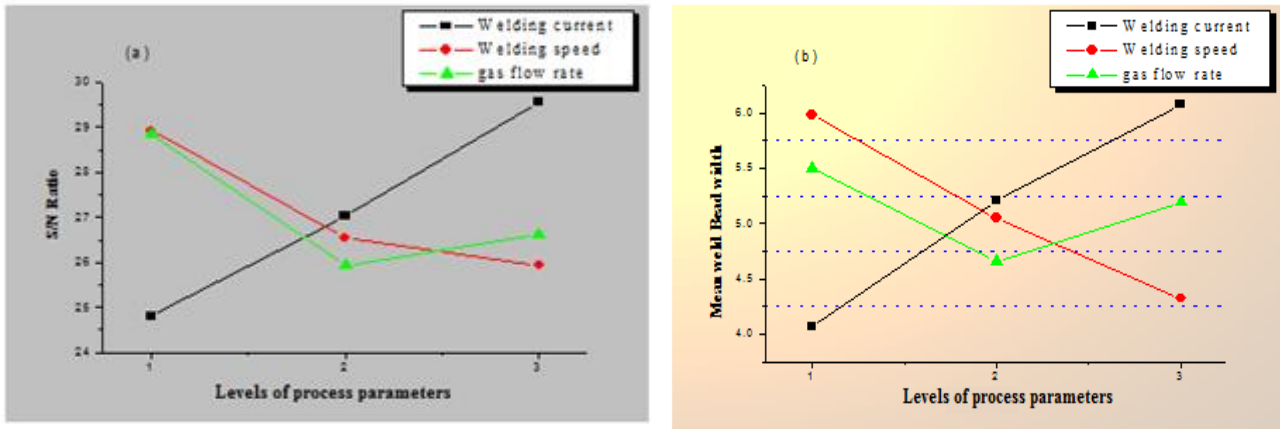
Figure 3. The average effect response for factors of the L9 (OA), (a) S/N ratio. (b) Weld bead width.
