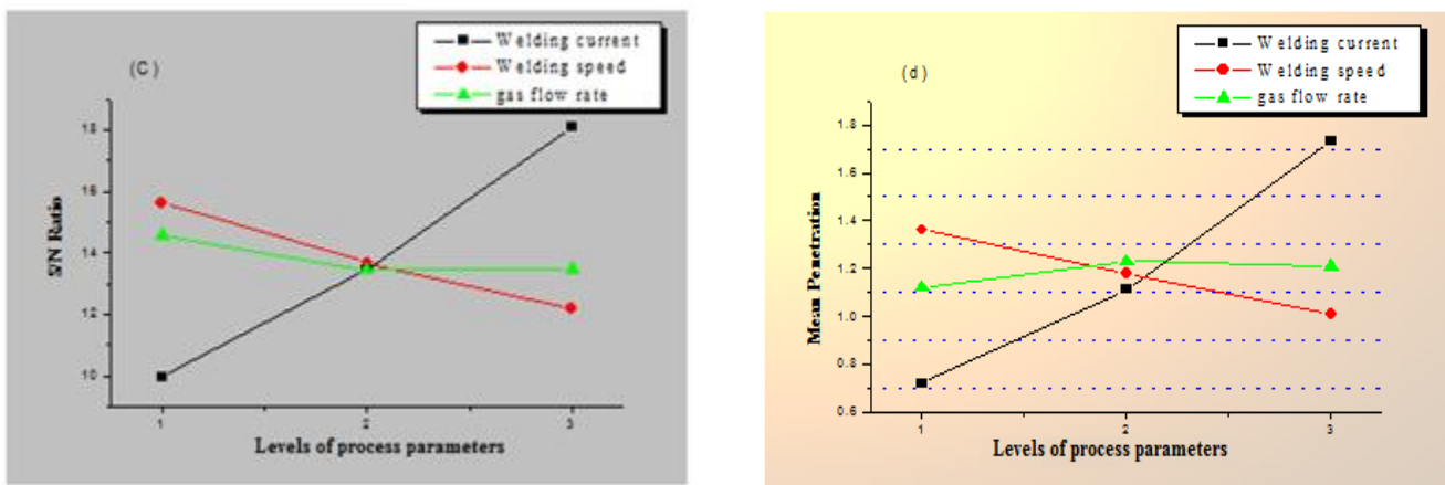
Figure 4. The average effect response for factors of the L9 (OA), (c) S/N ratio. (d) Penetration.
